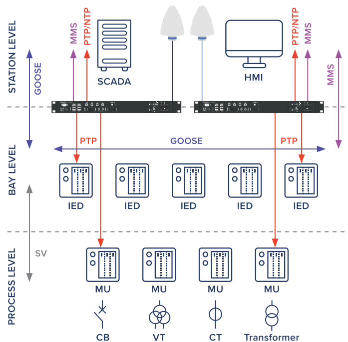
Functioning of communication protocols in IEC 61850
