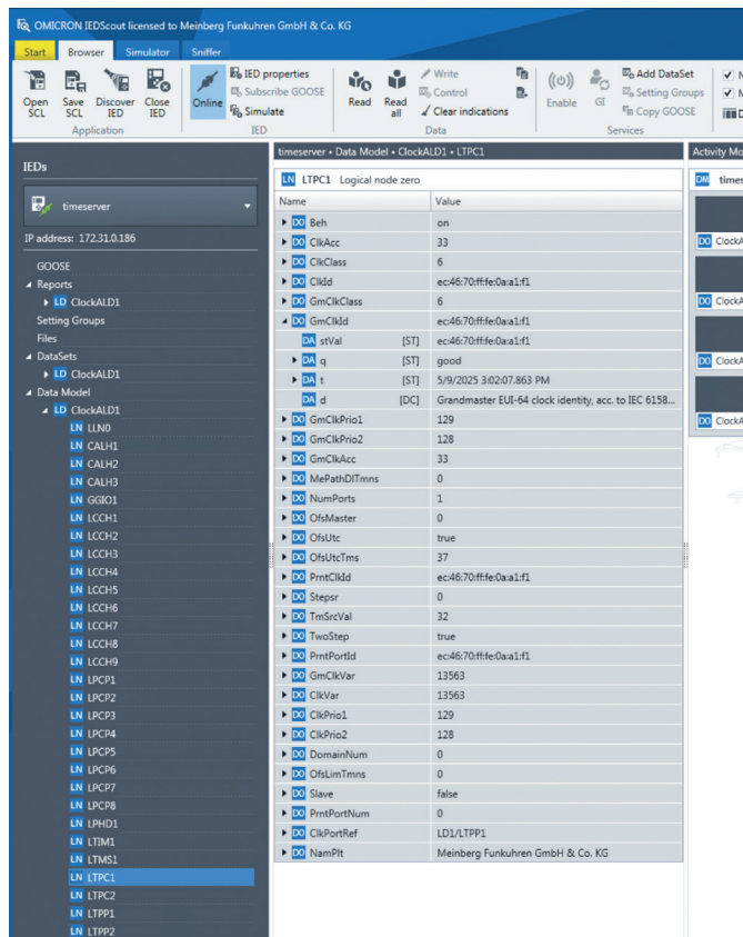
Omicron IED Scout Connected as a client to Meinberg MMS Server
